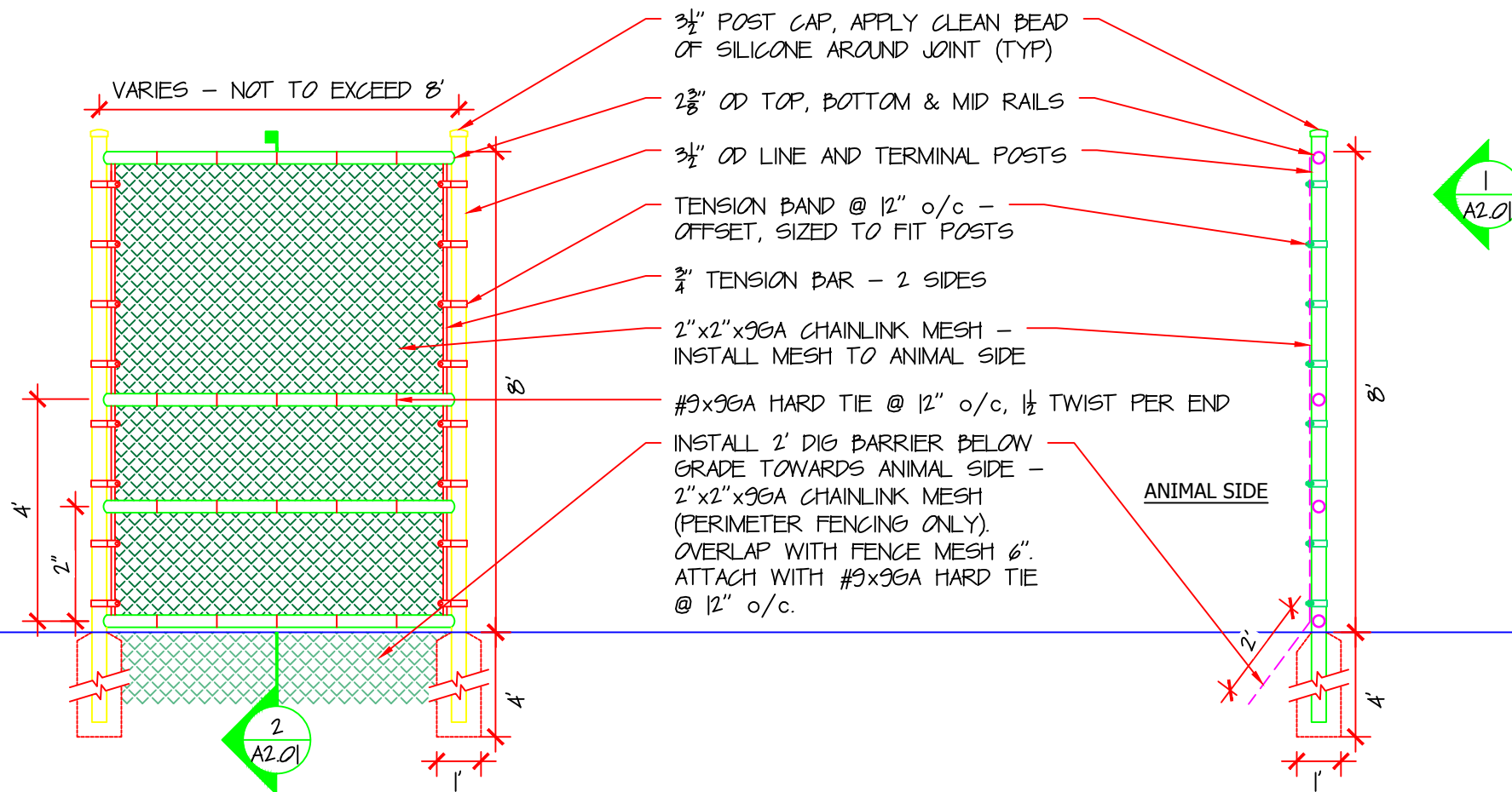
1 ENCLOSURE FENCE ELEVATION (TYPICAL) SCALE: 3/8" = 1'-0"
